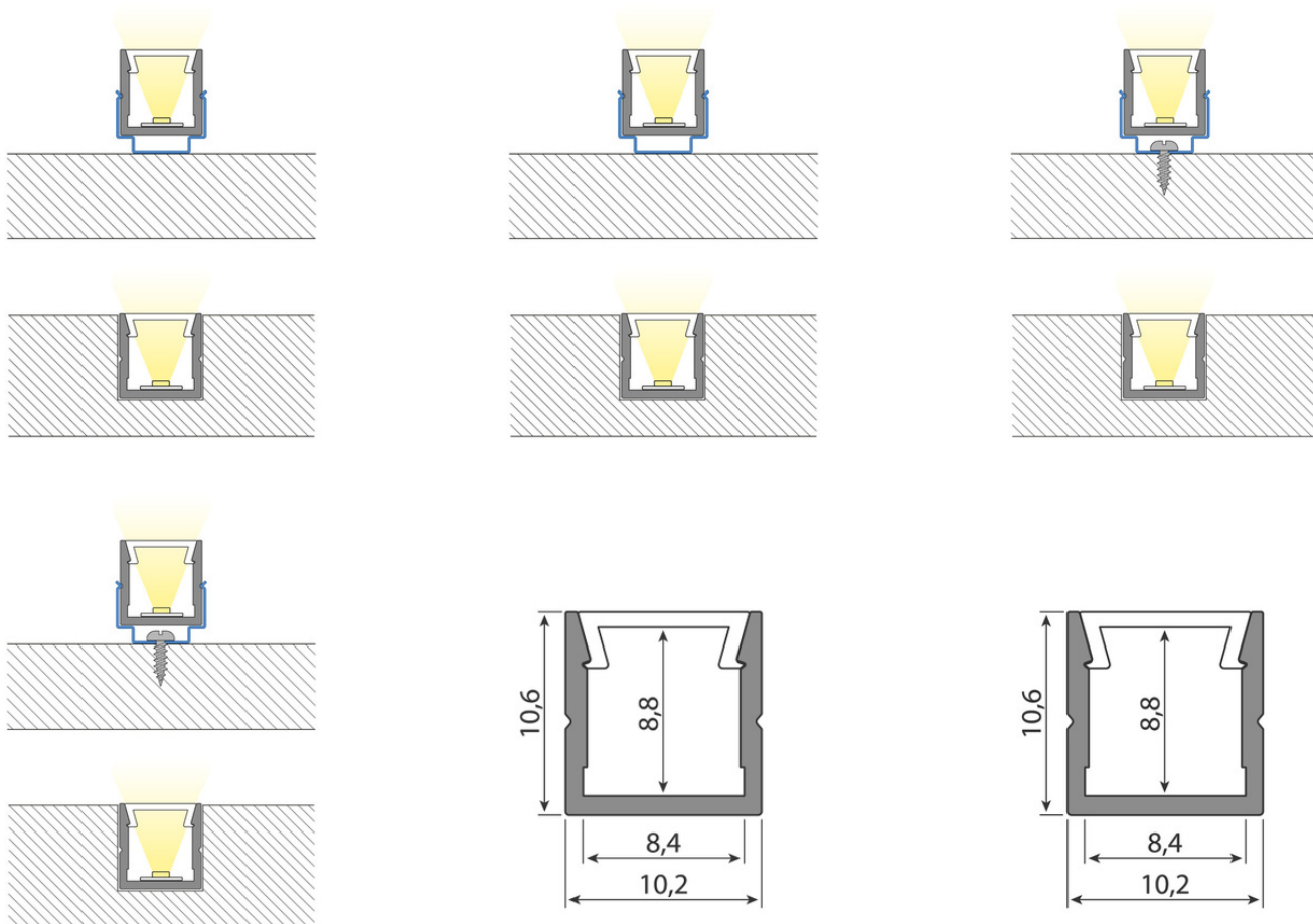
ML-762.329.74.0
