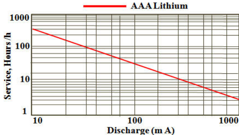
Working life at different discharge rates Discharge to 1.0V typical characteristics (25°C)
