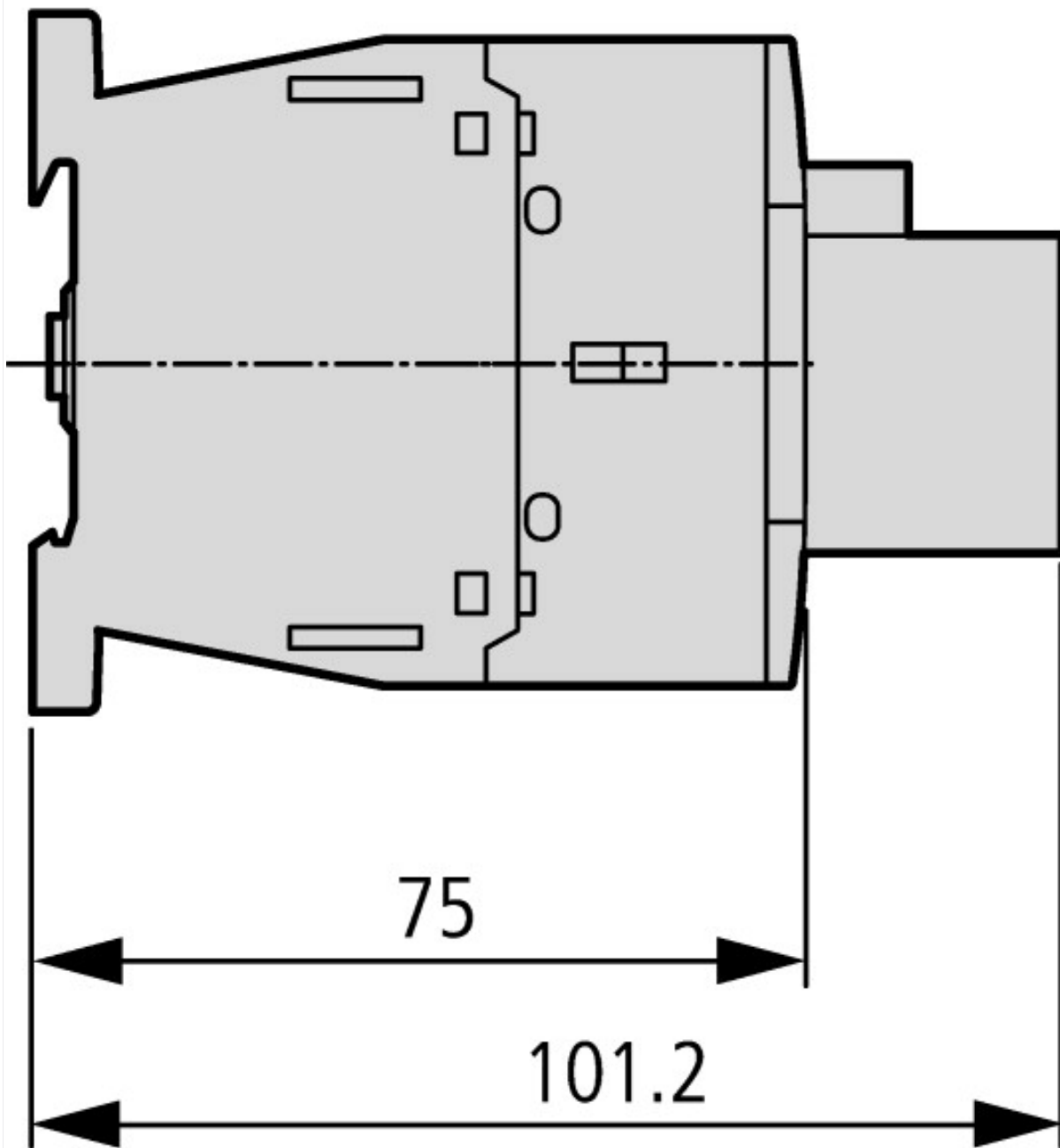
DILM12-XMSM
