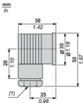
(1) Pg 11 cable gland
