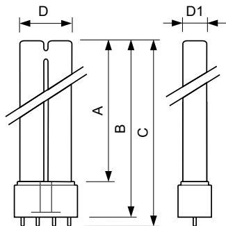
PL-L 24W/827/4P
