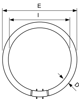
TL5-C 60W/840
